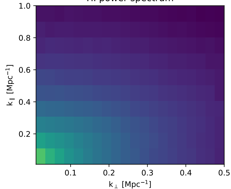
HI power spectrum
