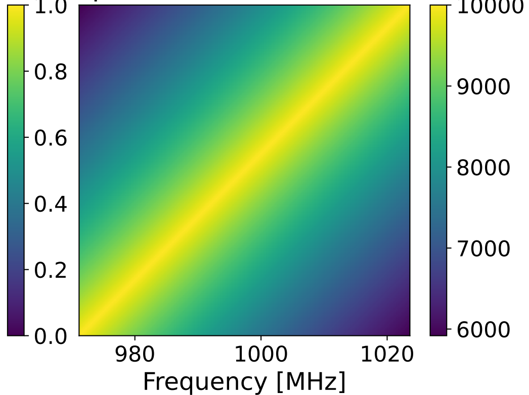
Exp ( \sigma = 100 , l = 100 MHz)
