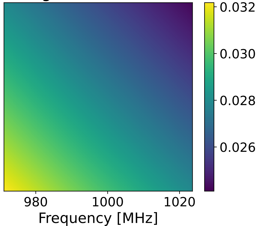
Foreground covariance
