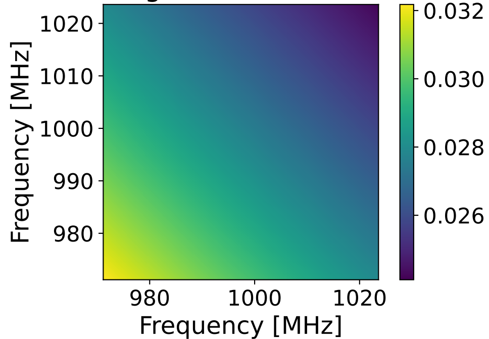
Foreground covariance
