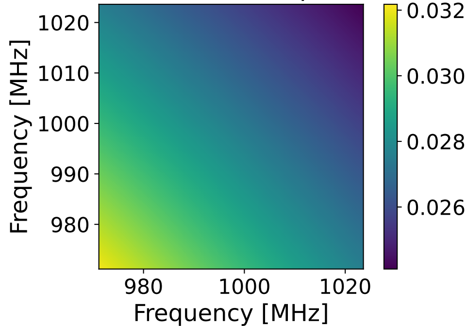
RBF ( l = 400 MHz, \gamma = -2.7 )
