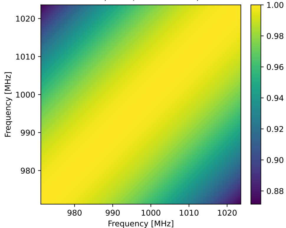
RBF ( \sigma = 1 , l = 100 MHz)
