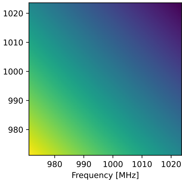
Total signal
