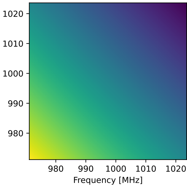
Foreground
