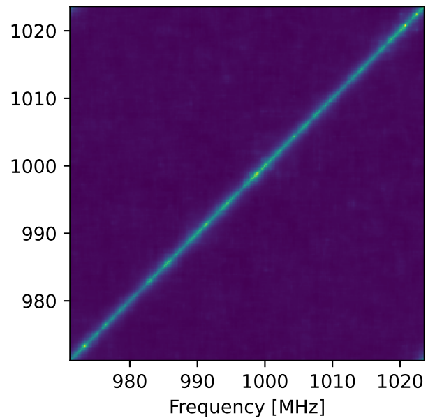
HI signal
