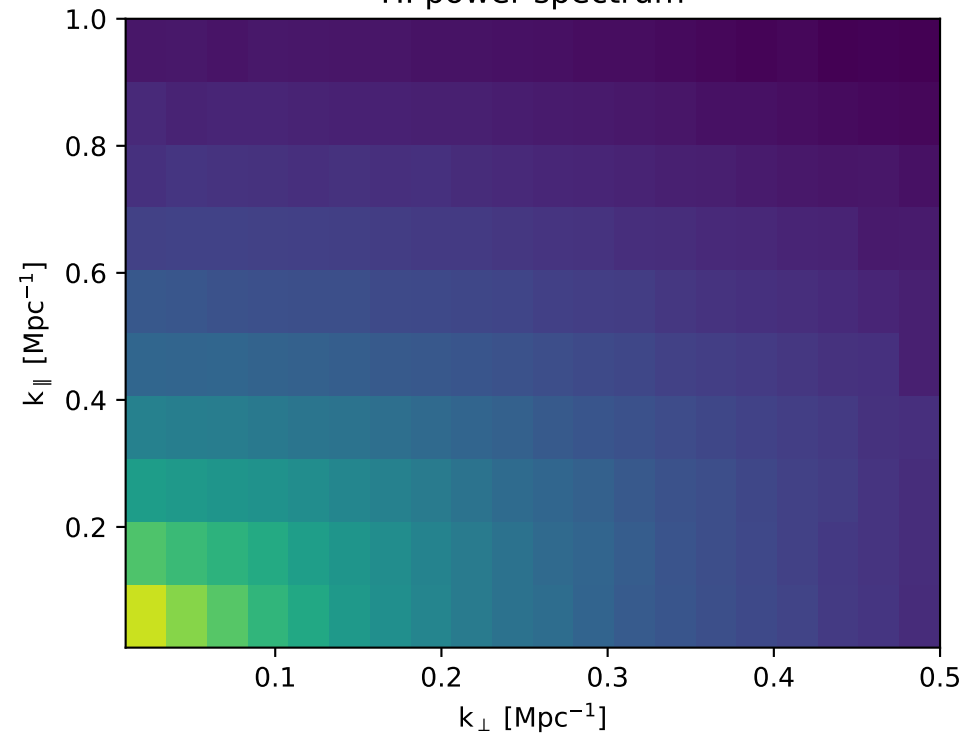
HI power spectrum
