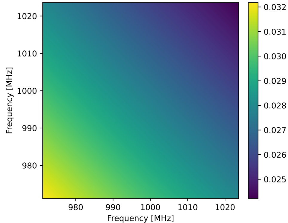
Foreground covariance
