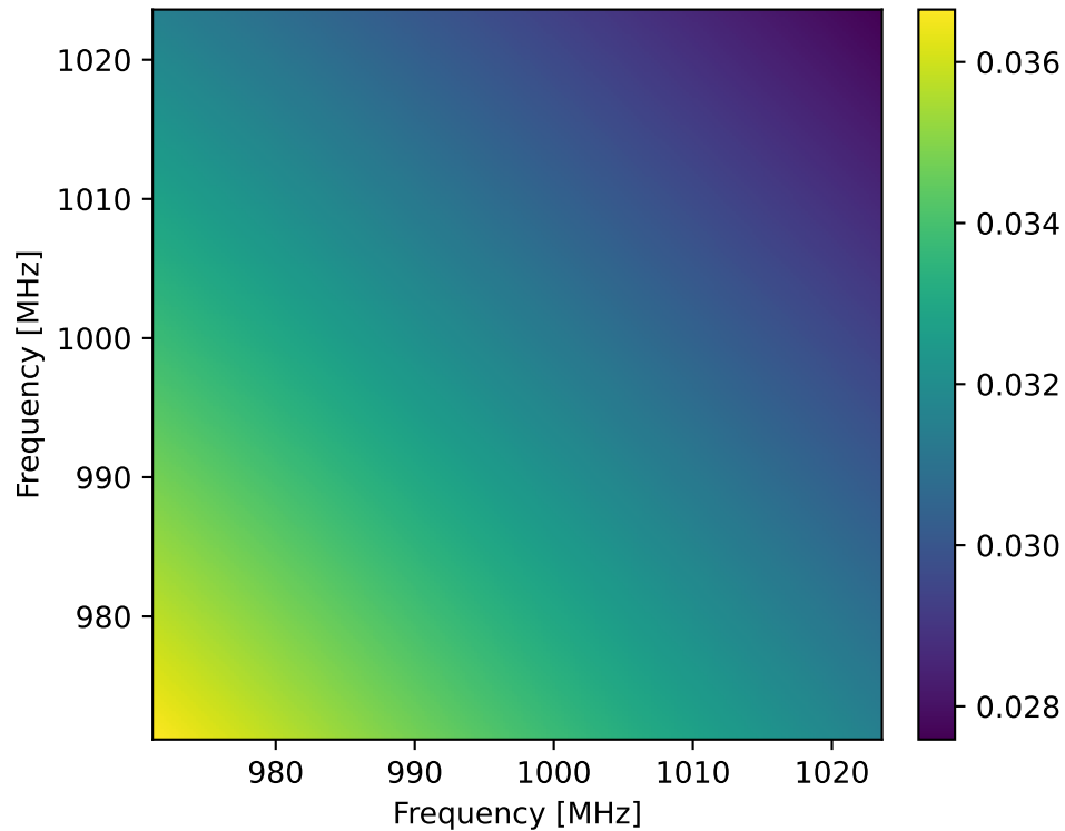
Best fit foreground kernel
