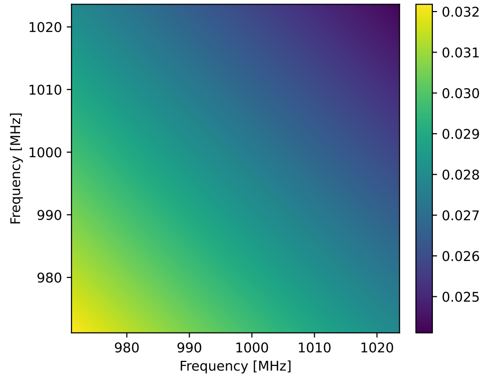
Foreground covariance
