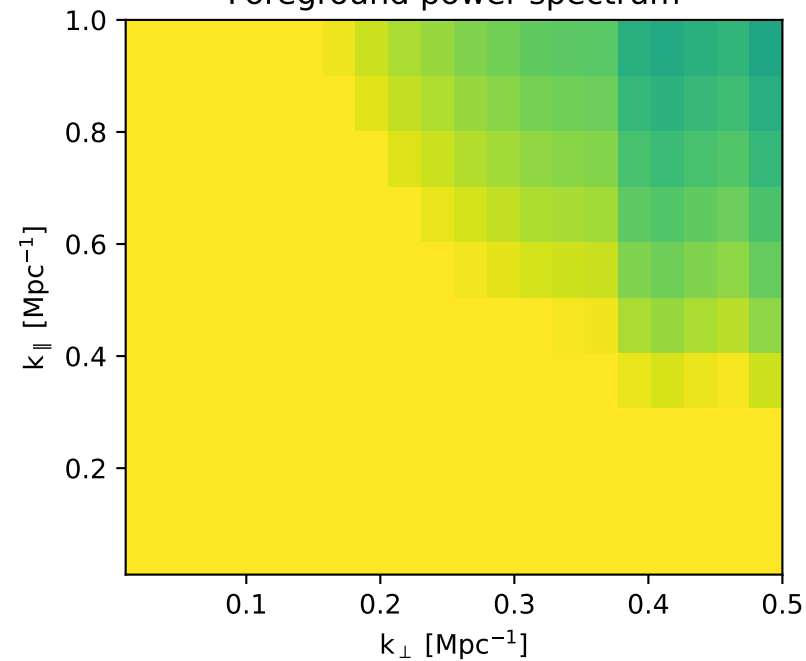
Foreground power spectrum
