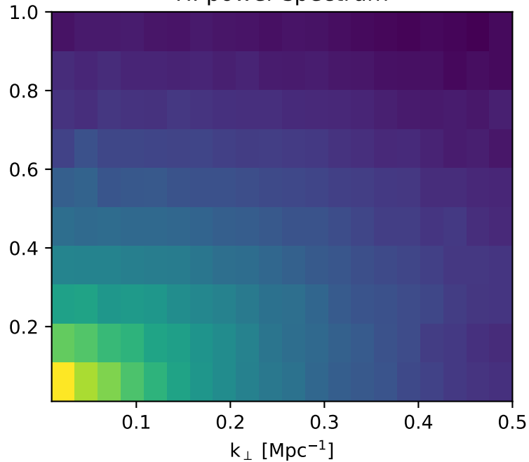
HI power spectrum
