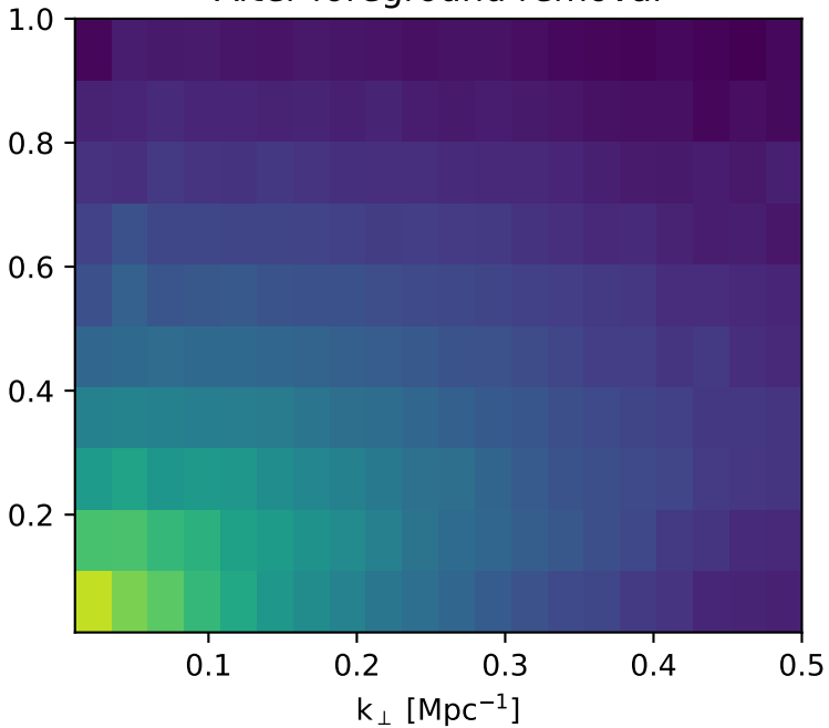
After foreground removal
