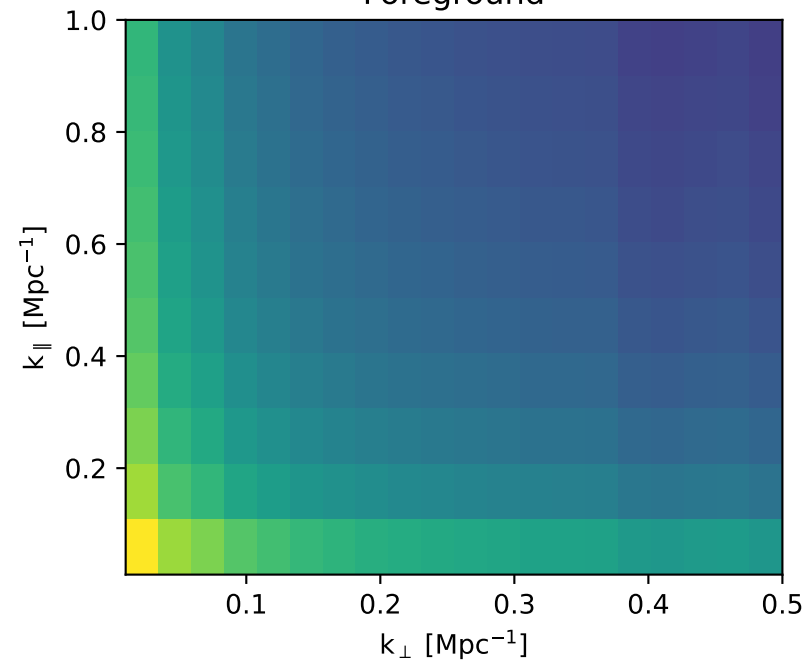
Foreground
