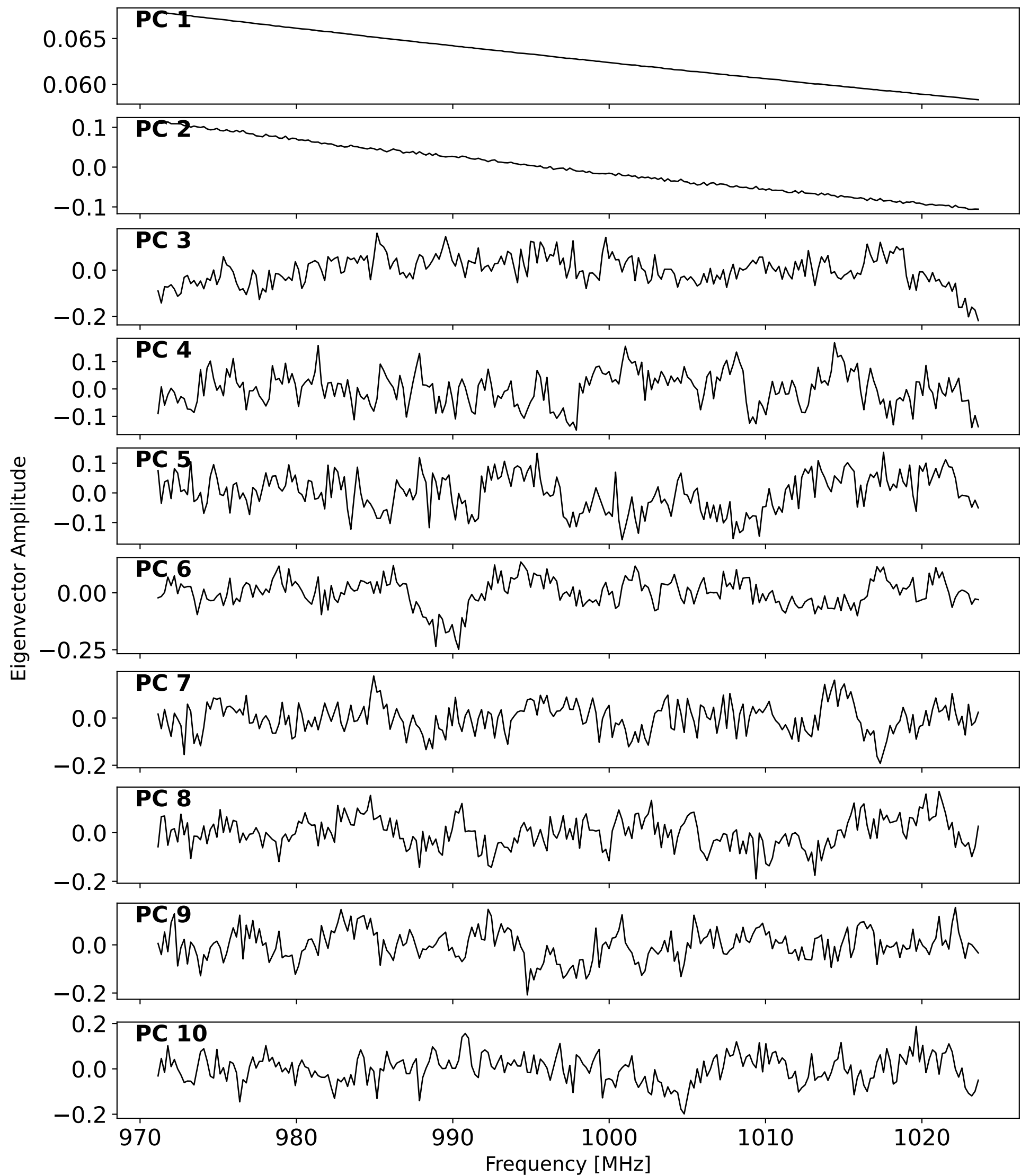
First 10 PCA Eigenvectors (Foreground Modes)
