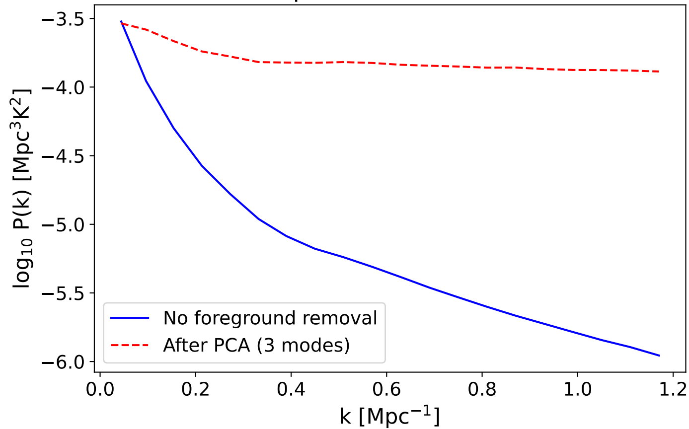
1D Power Spectrum — PCA Benchmark
