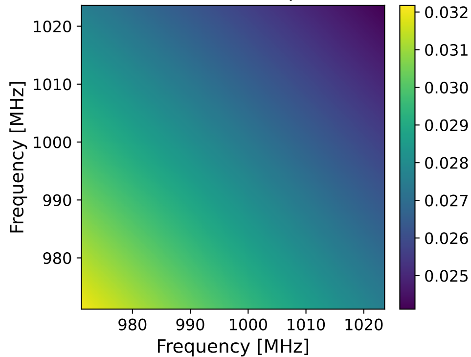
RBF ( l = 400 MHz, \gamma = -2.7 )
