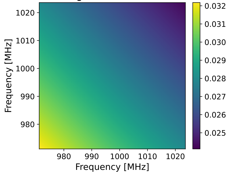
Foreground covariance
