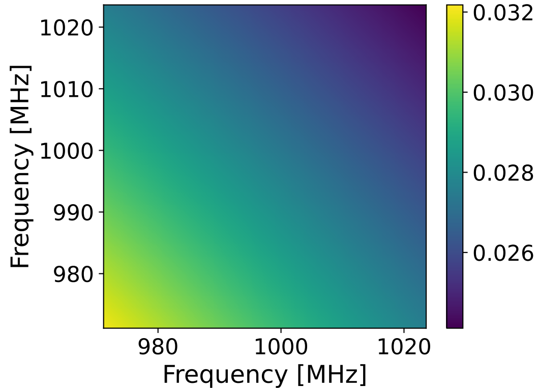
RBF ( l = 400 MHz, \gamma = -2.7 )
