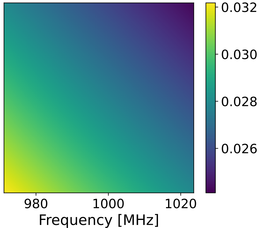
Foreground covariance
