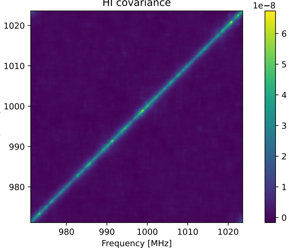
HI covariance
