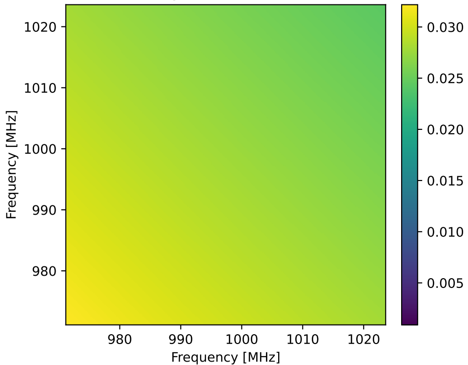
Foreground covariance
