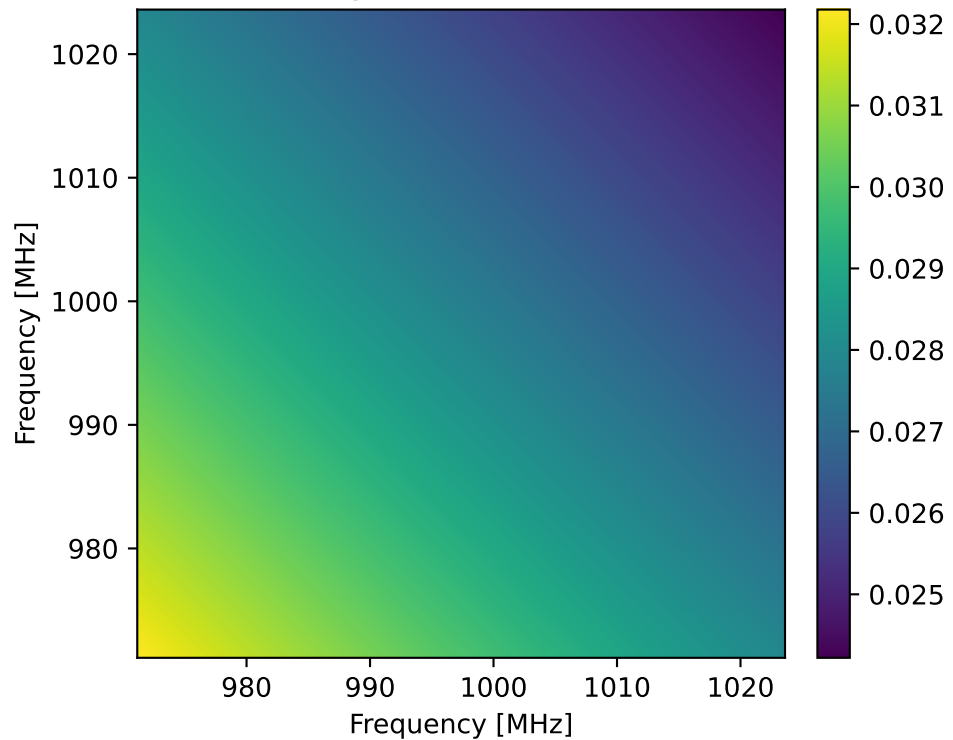
Foreground covariance
