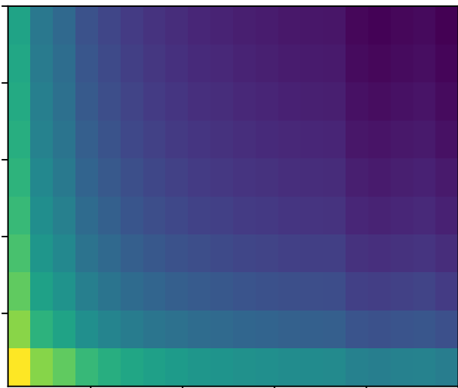
Foreground power spectrum
