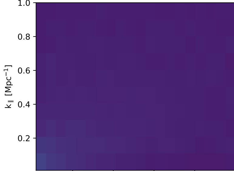
After foreground removal
