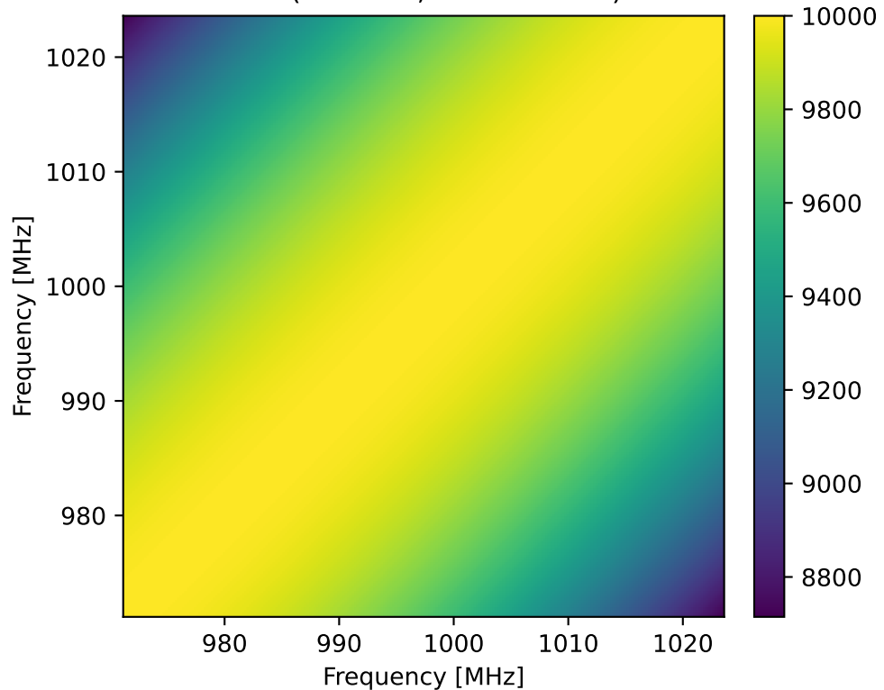
RBF ( \sigma = 100 , l = 100 MHz)
