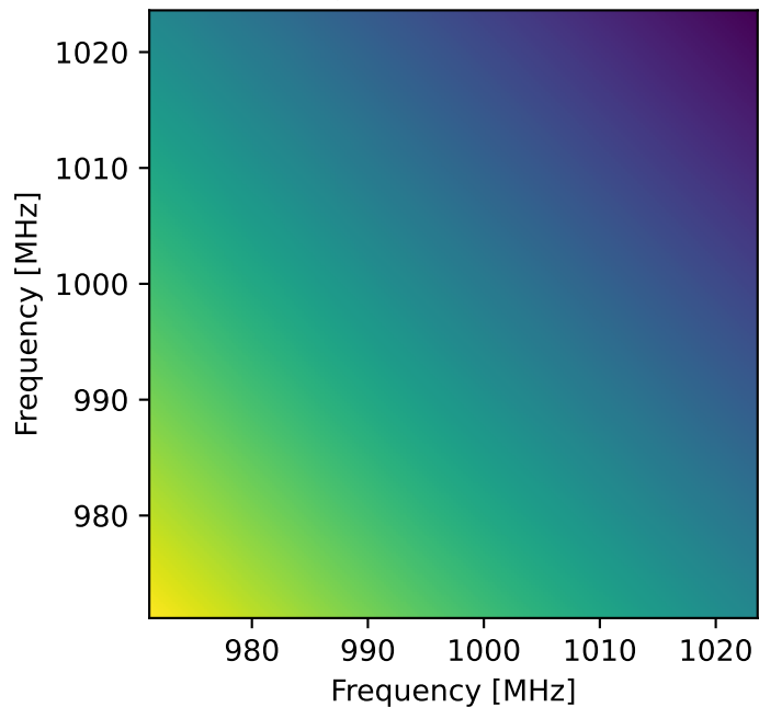
Foreground covariance
