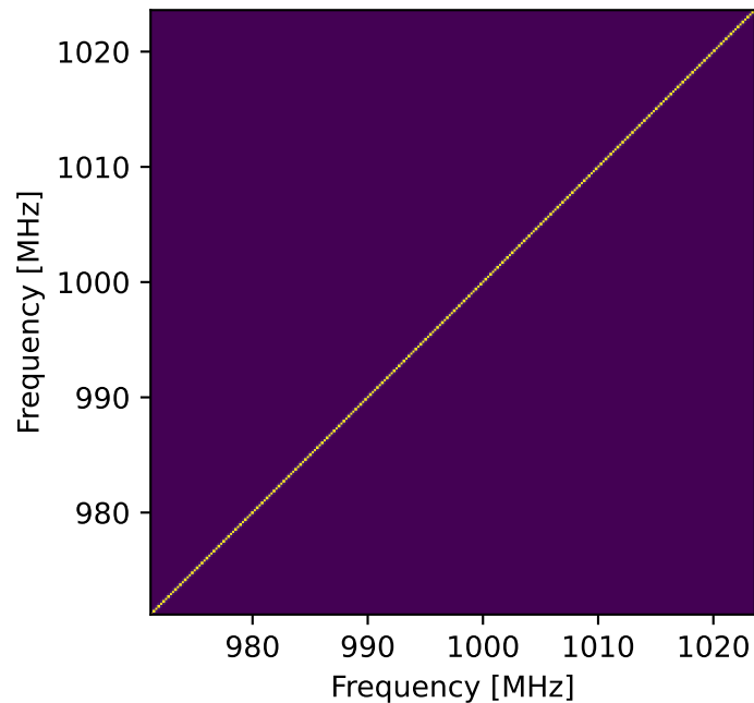
Fitted HI + noise kernel
