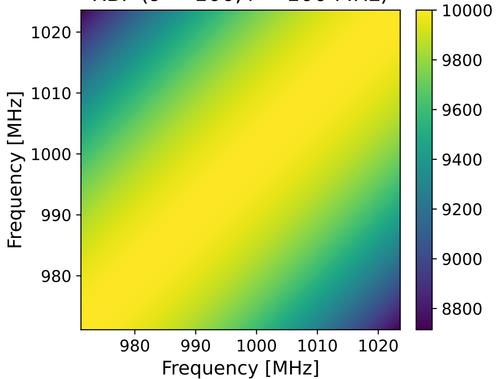
RBF ( \sigma = 100 , l = 100 MHz)
