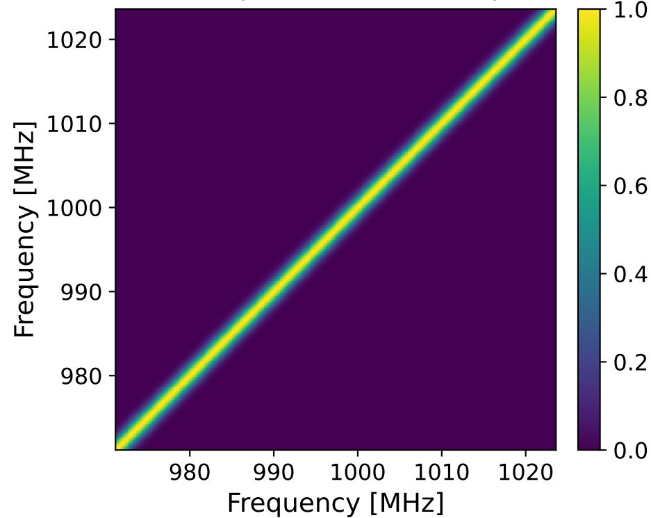
RBF ( \sigma = 1 , l = 1 MHz)
