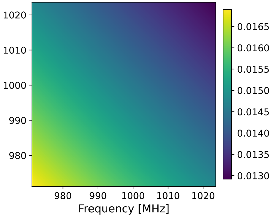
Foreground covariance
