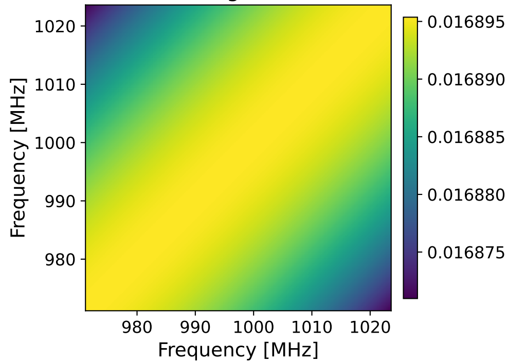
Best fit foreground kernel
