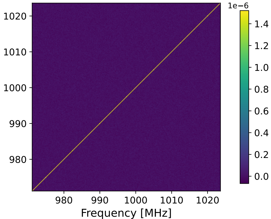
Noise covariance
