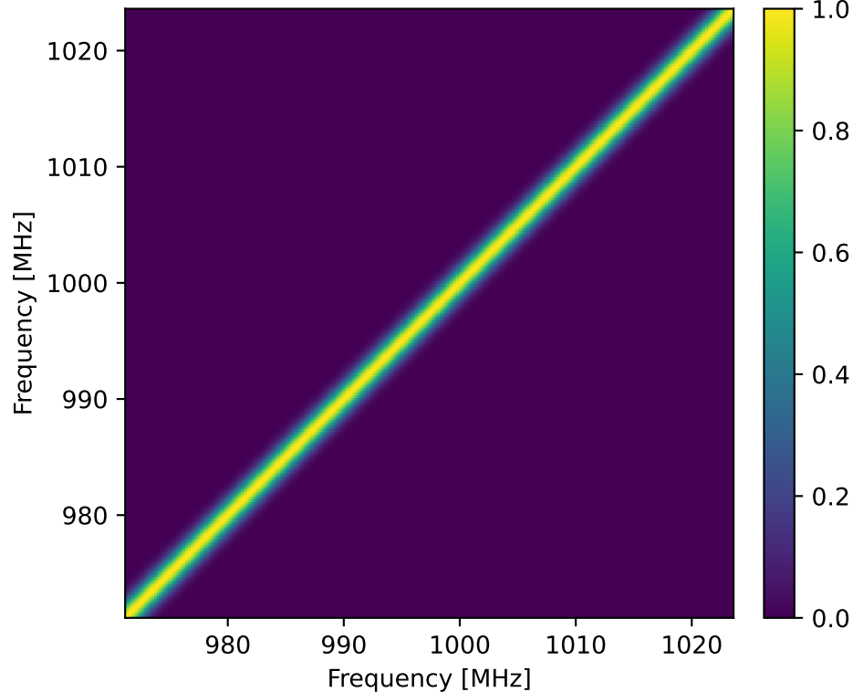
RBF ( \sigma = 1 , l = 1 MHz)
