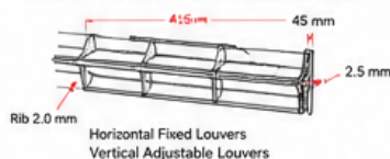
WINDOW AC FRONT GRILL (SECTION VIEW)
