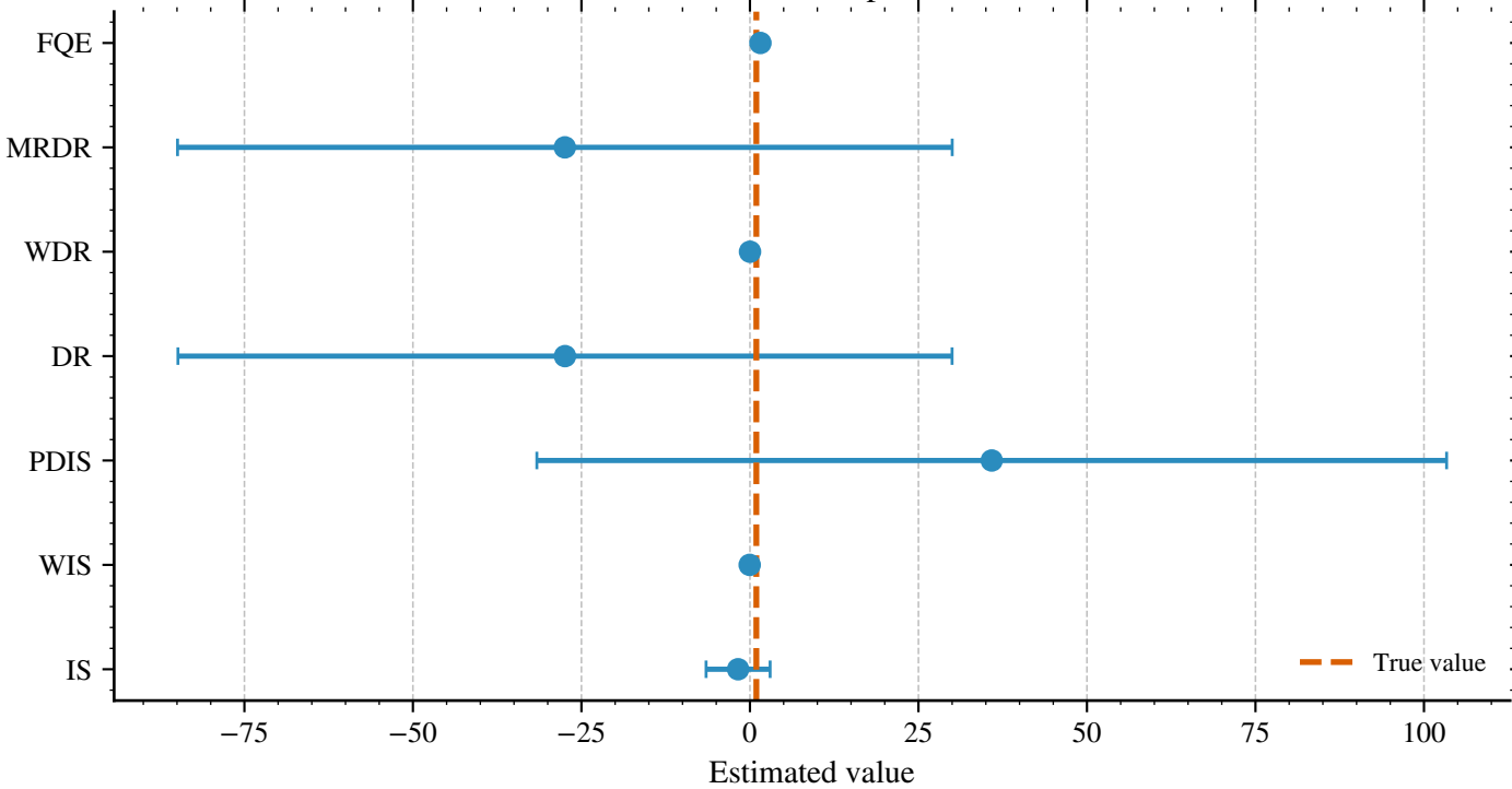
Estimator Comparison
