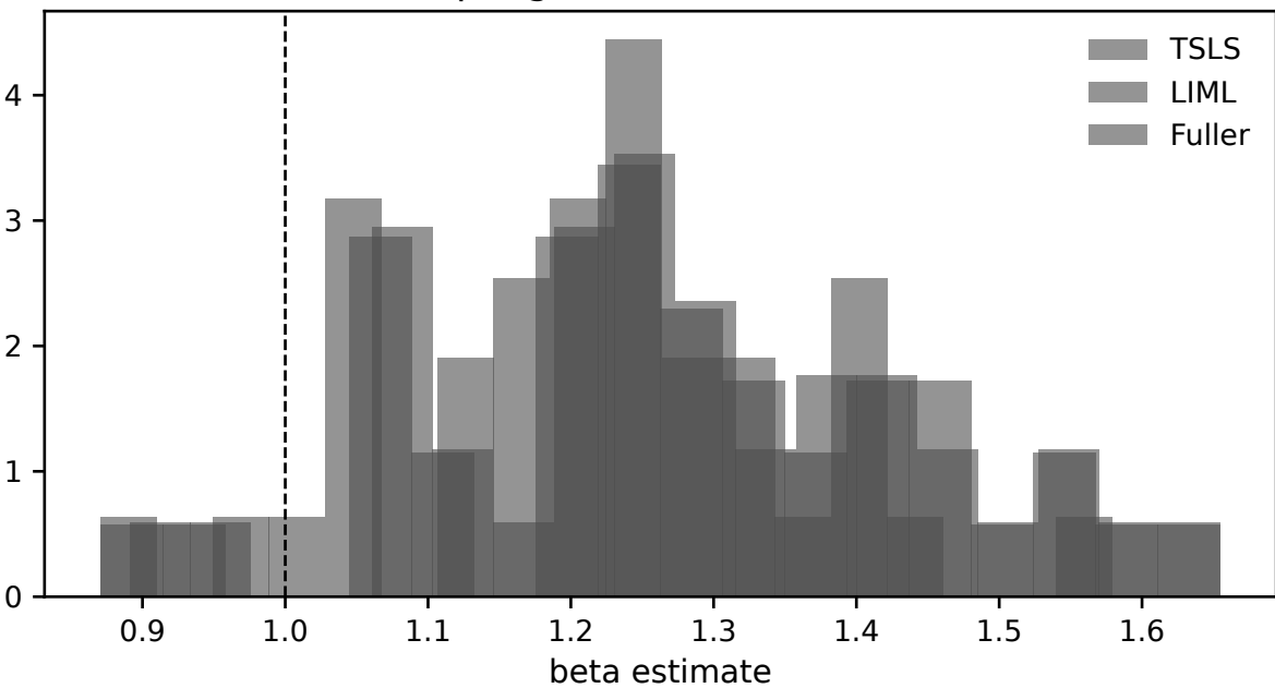
Sampling distributions (k=20)
