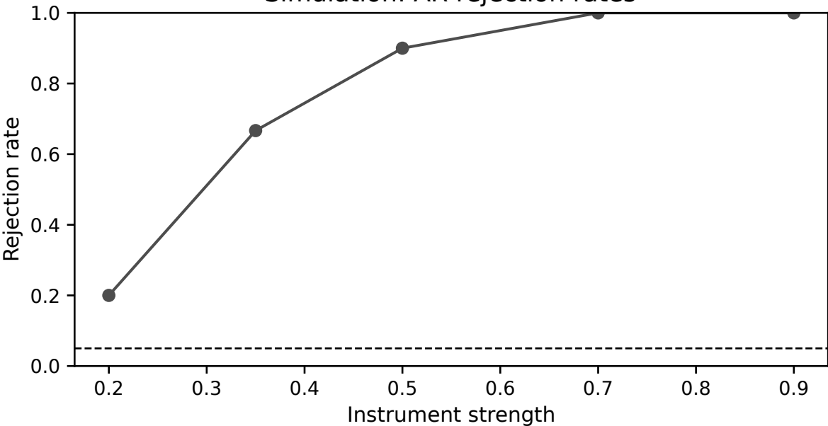
Simulation: AR rejection rates
