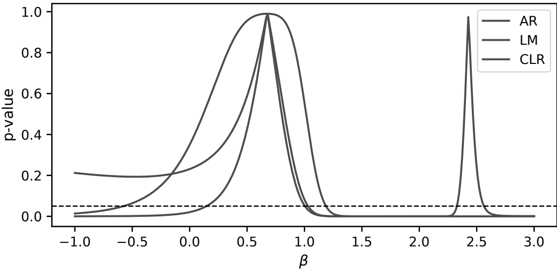
AR/LM/CLR p-value curves
