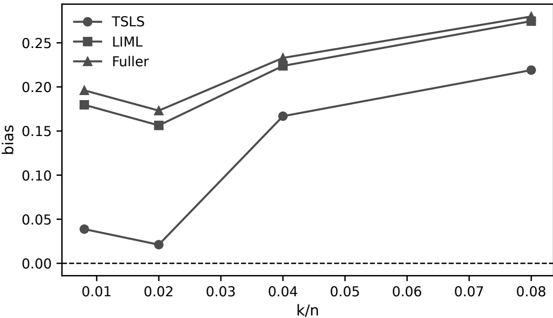
Estimator bias vs k/n
