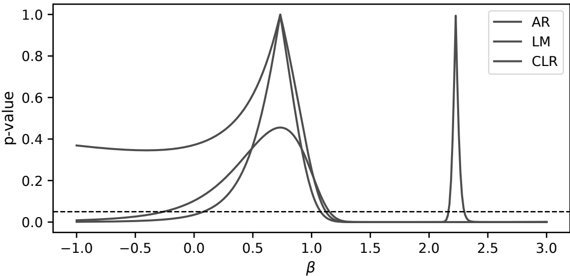
Weak-IV p-value curves
