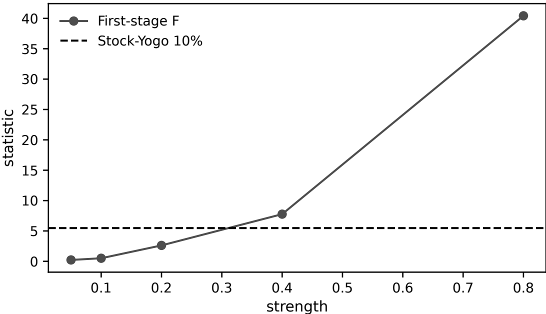
Stock-Yogo threshold overlay
