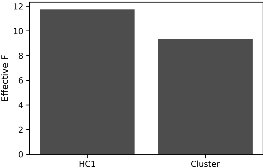
Instrument strength under clustering
