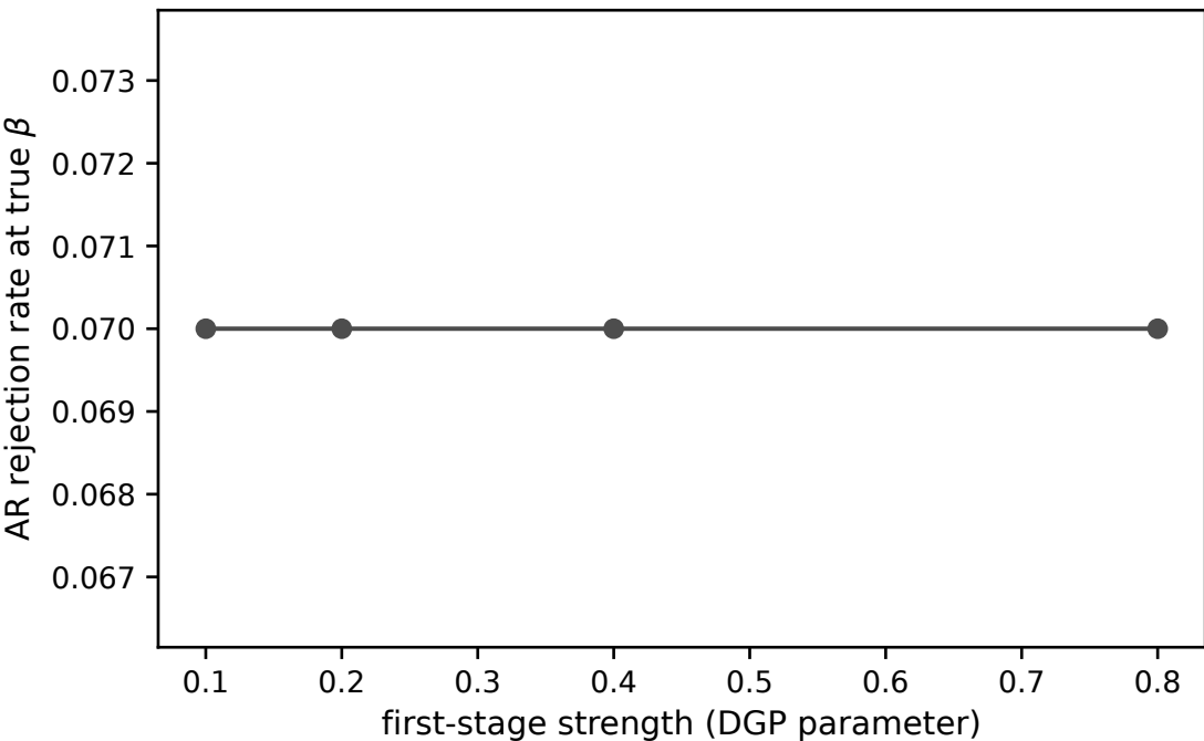
Monte Carlo illustration (should be near size)
