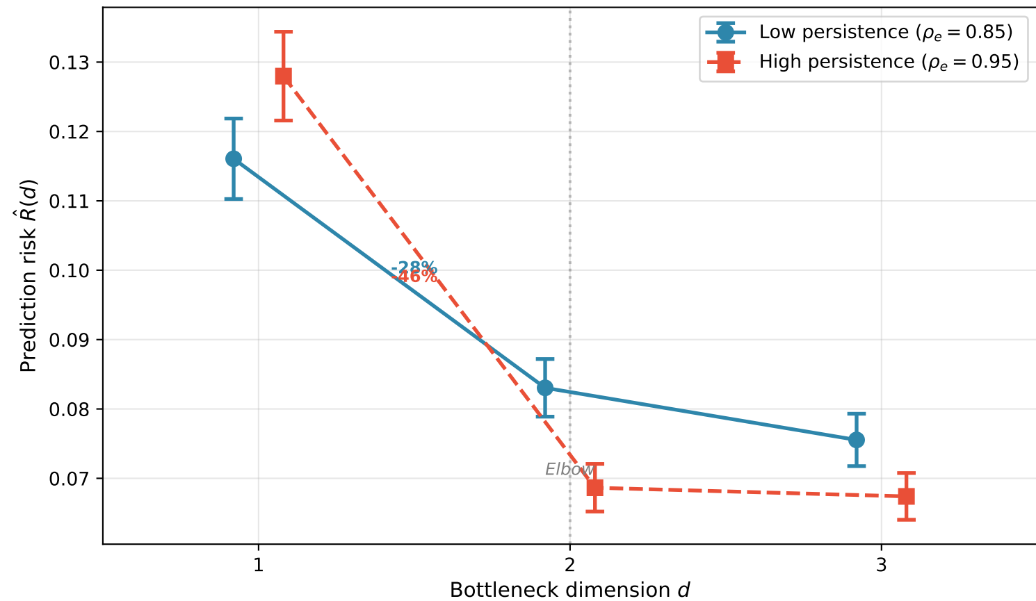
Prediction Risk vs. Bottleneck Dimension
