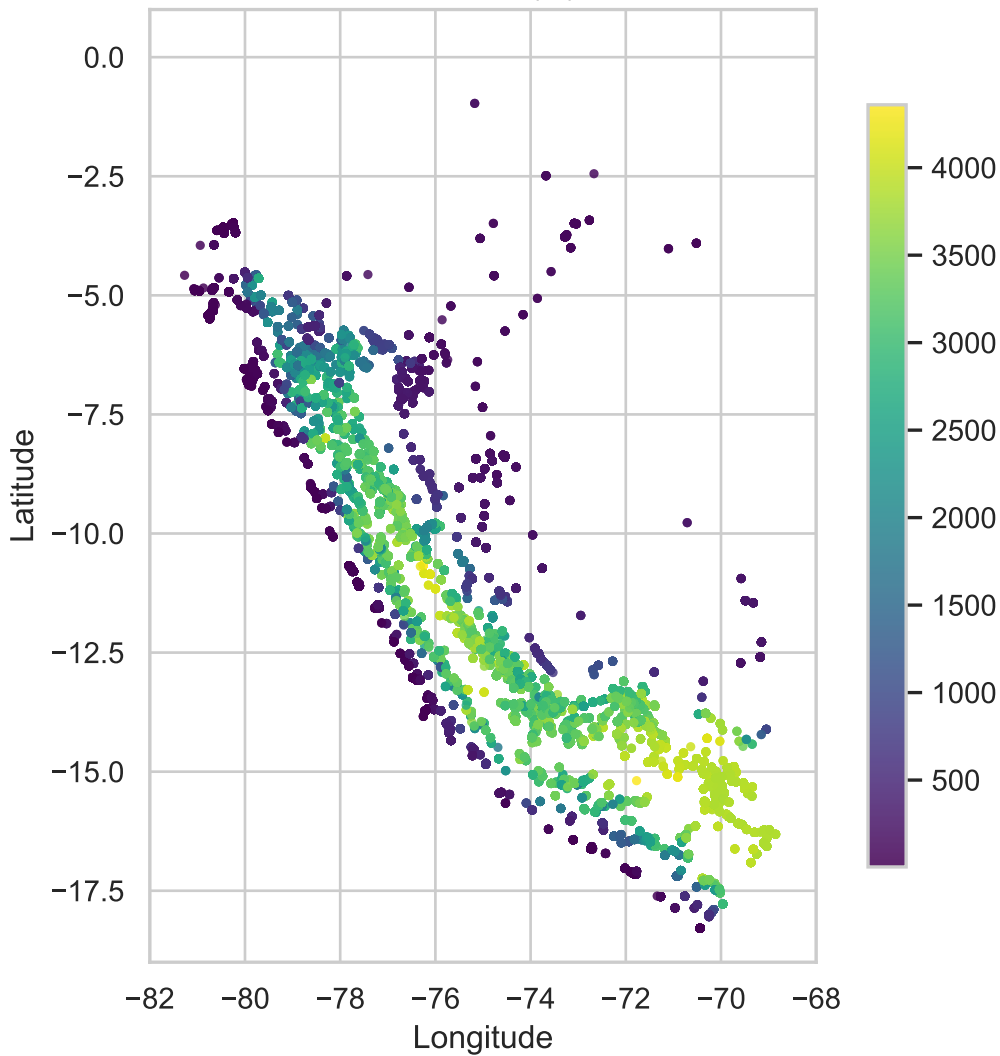
Elevation (m)
