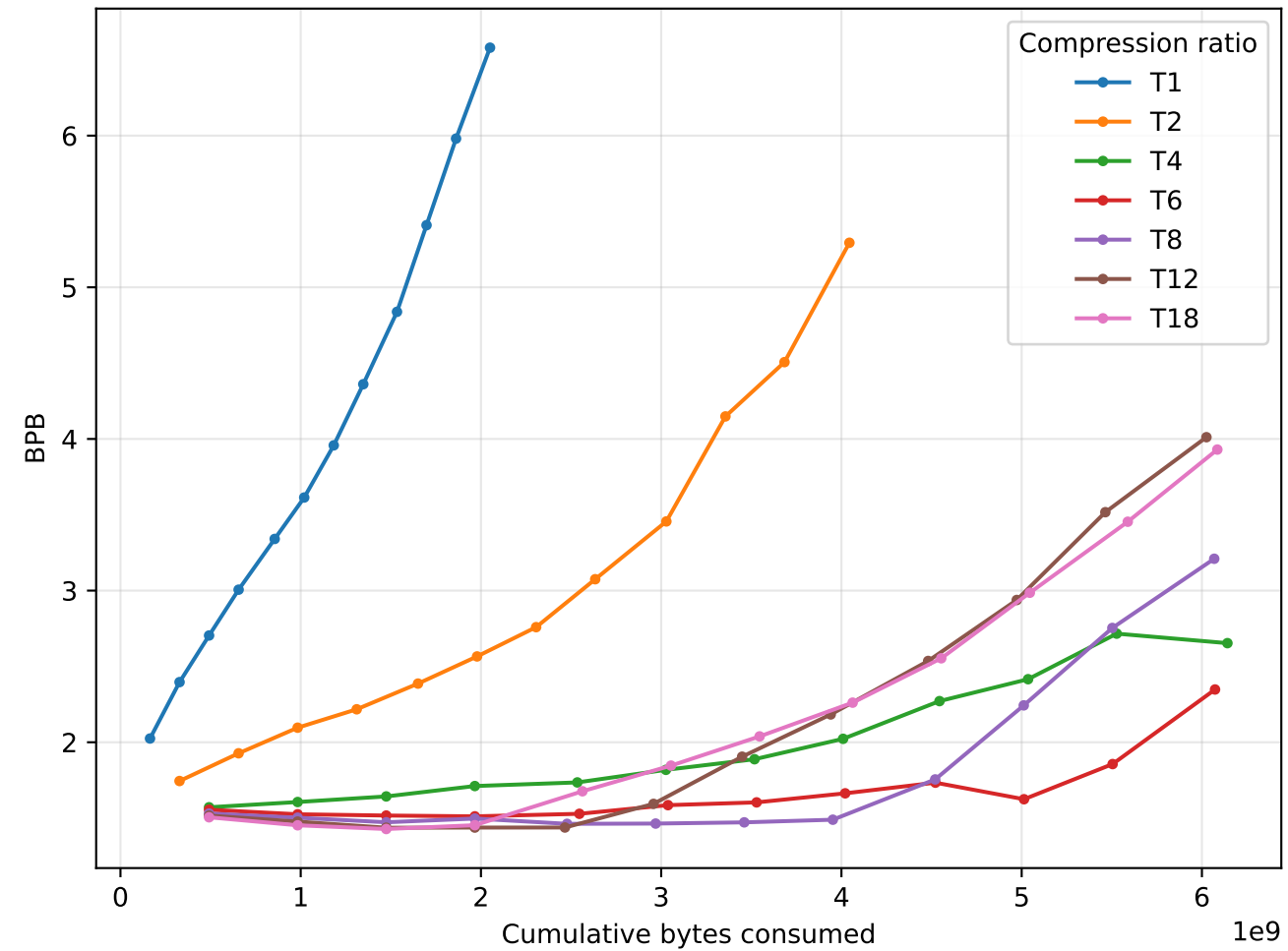
Eval BPB (FLORES English)
