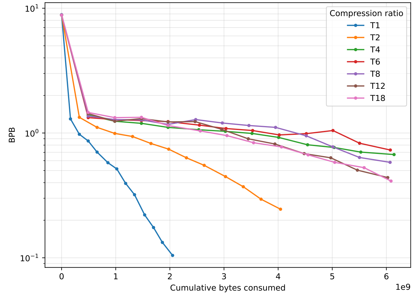
Training BPB (FineWeb)
