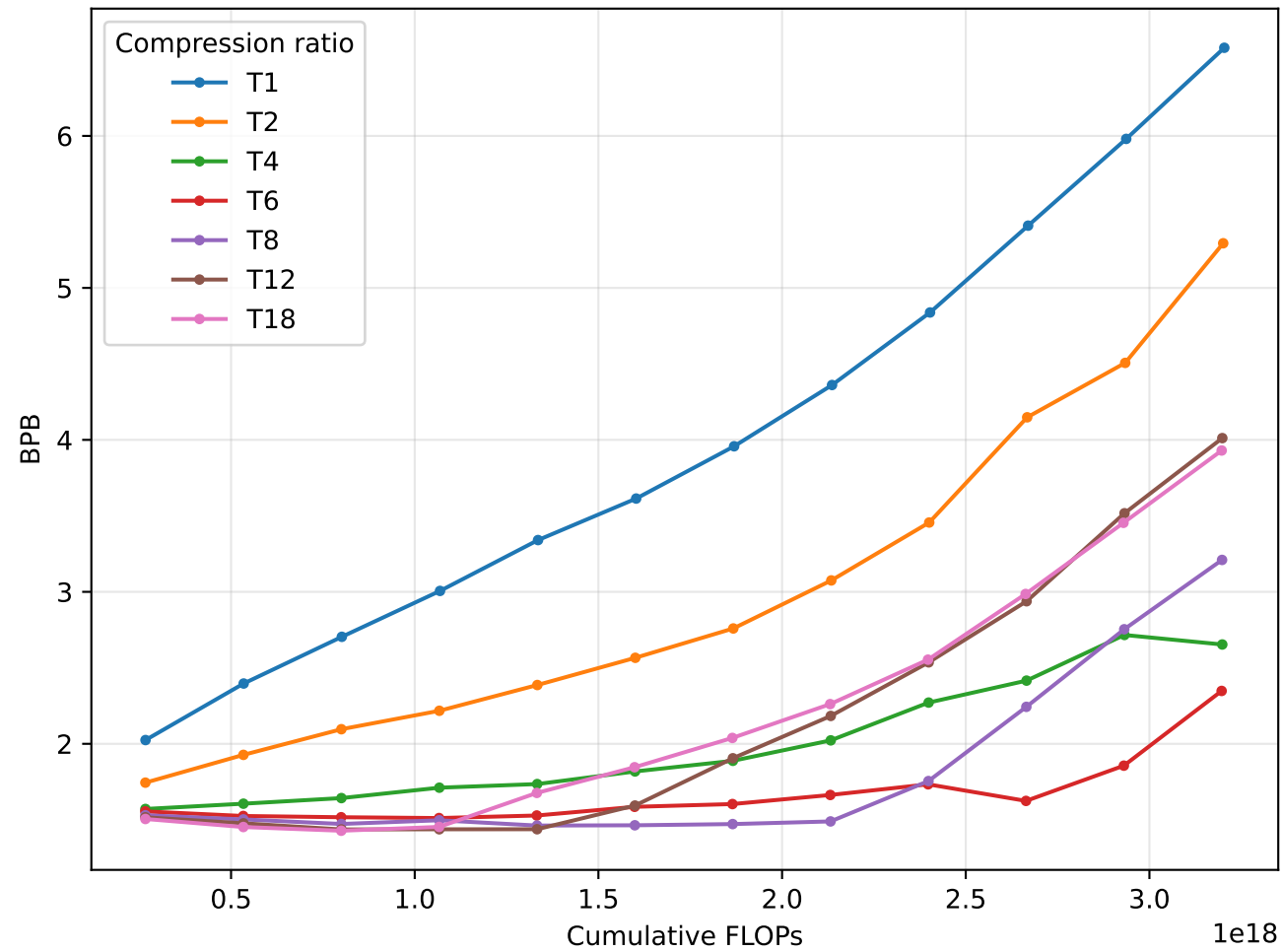
Eval BPB (FLORES English)
