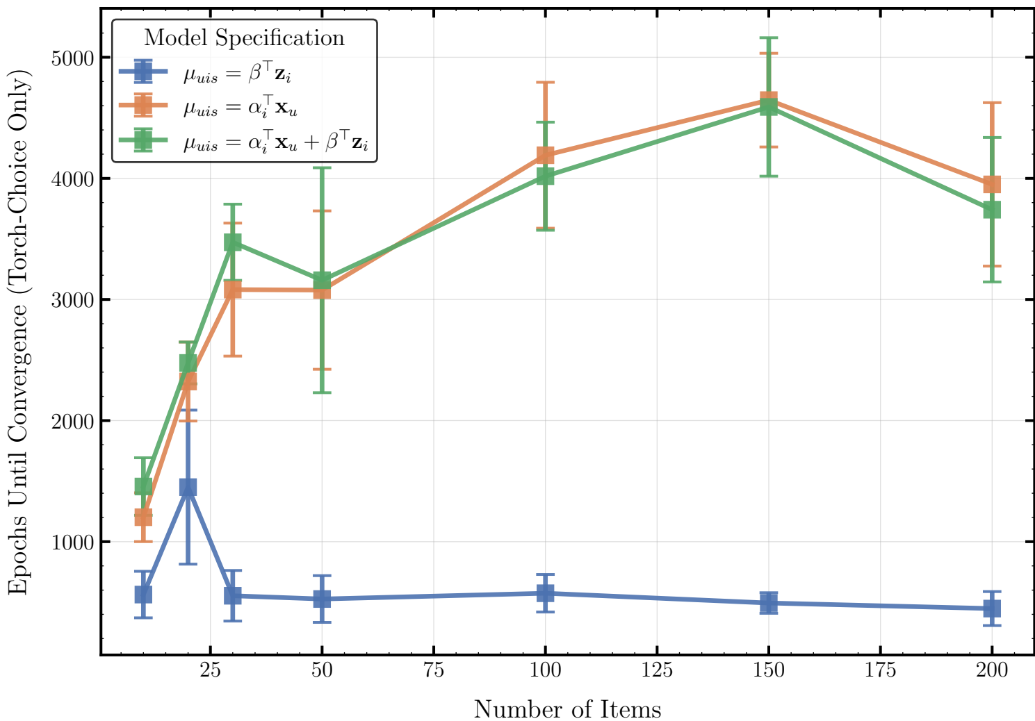
Torch-Choice Small Scale - Epochs Until Convergence
