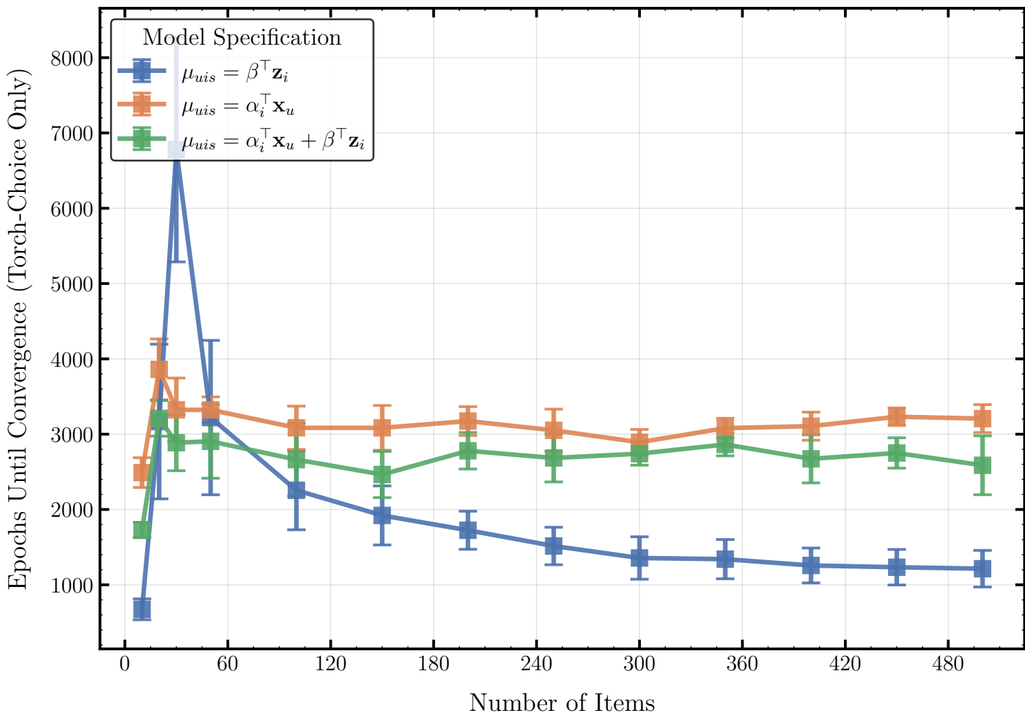
Torch-Choice Large Scale - Epochs Until Convergence
