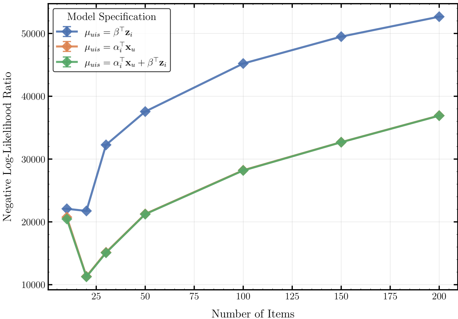
Torch-Choice Small Scale - Loss Benchmark
