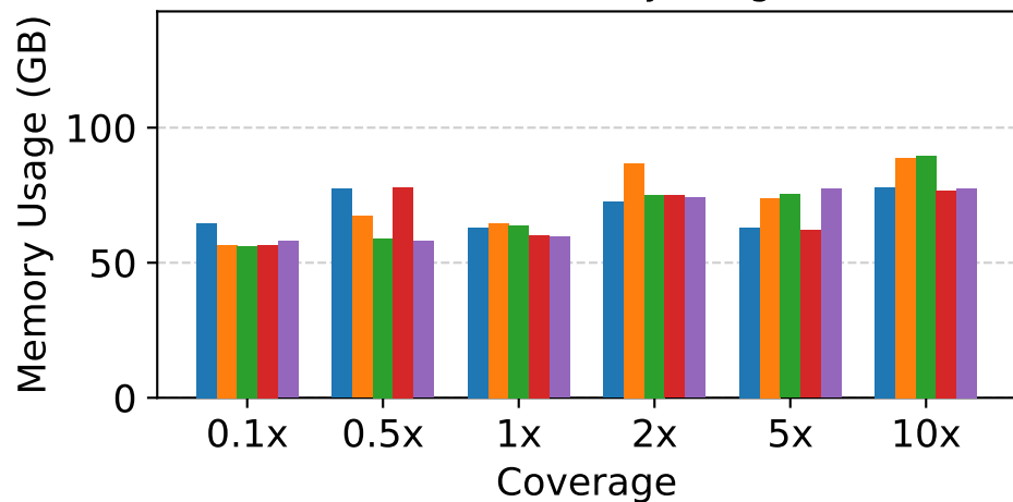
(C) ILP Memory Usage
