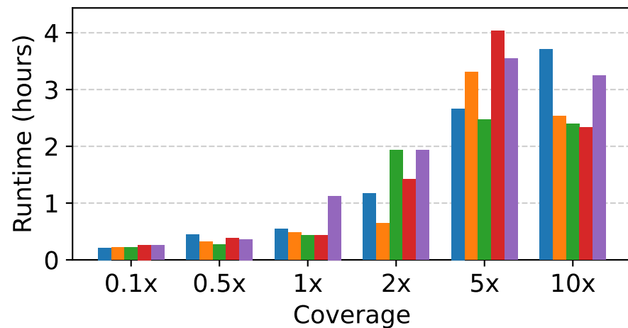
(A) MILP Runtime
