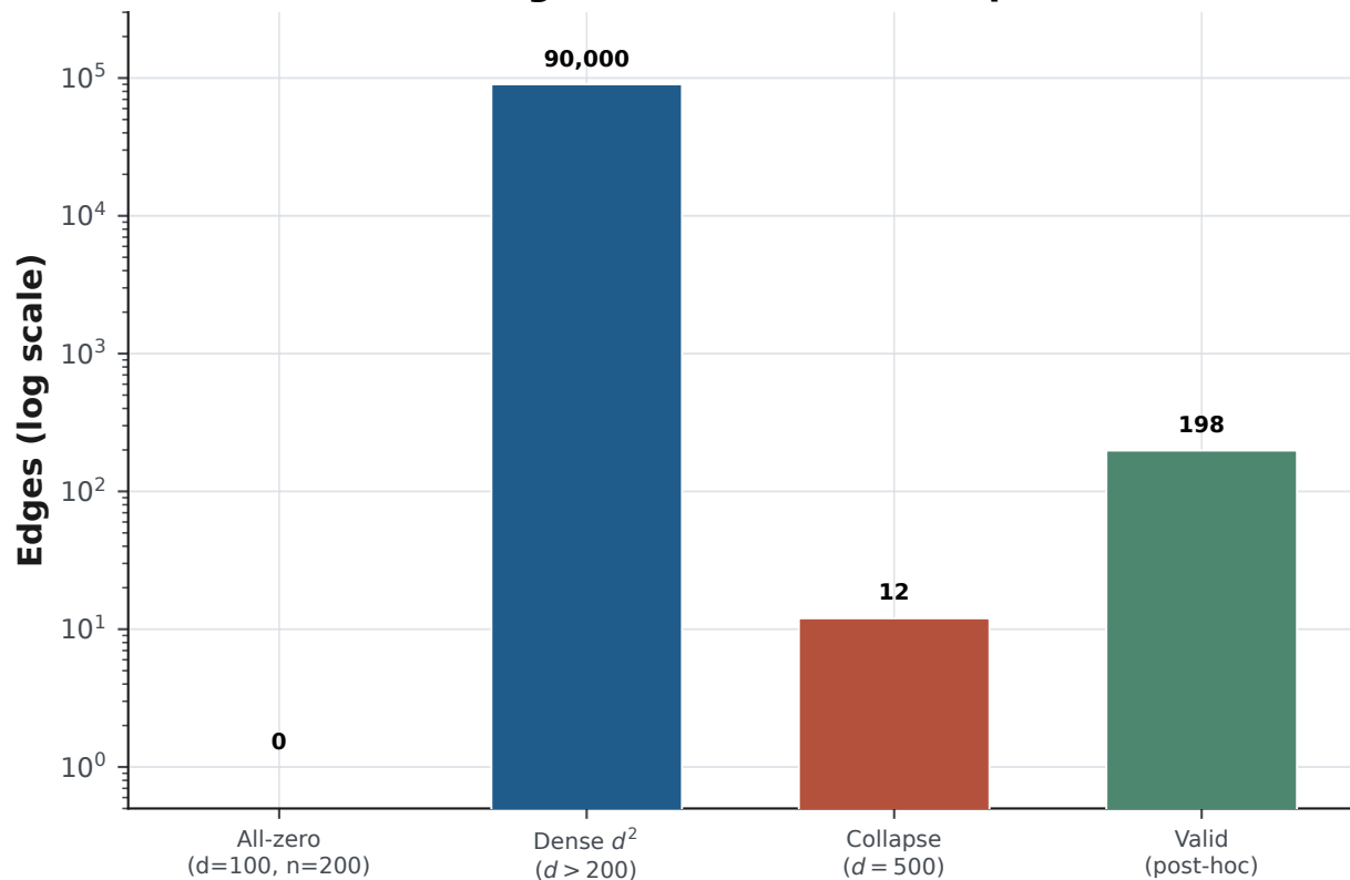
(b) Degenerate vs usable outputs
