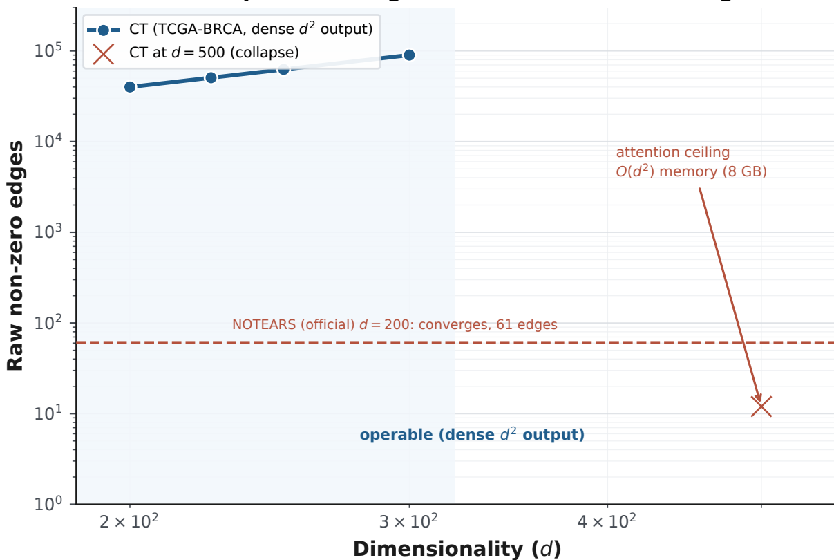
(a) Operable range and the attention ceiling
