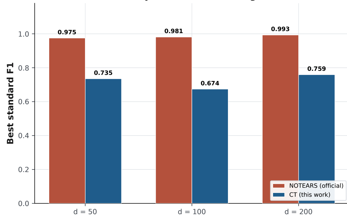
(b) Standard recovery: NOTEARS is stronger
