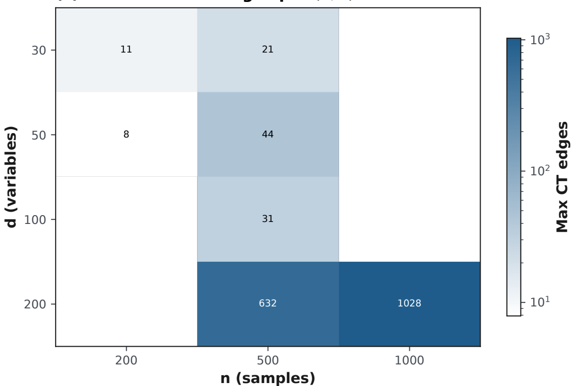
(c) Phase: max CT edges per ( d, n )
