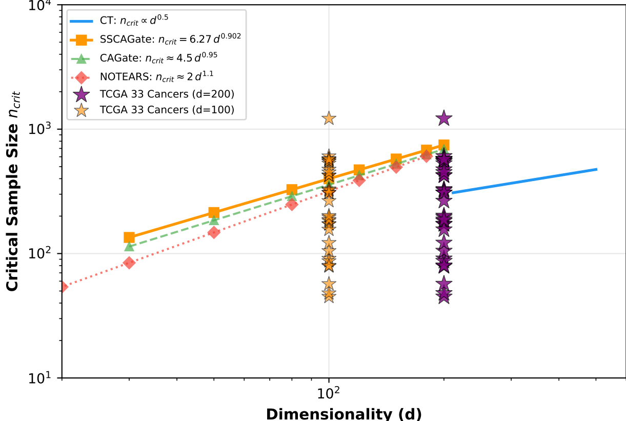
Scaling Laws: n_{crit}(d) = A \cdot d^\alpha
