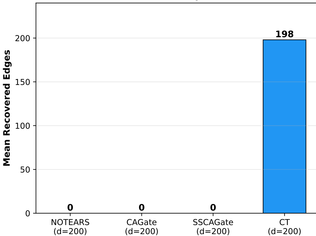
TCGA at d=200: Only CT is Viable
