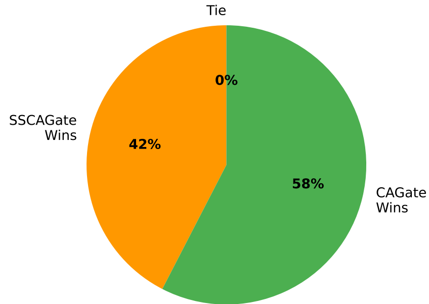
TCGA at d=100: Method Dominance (33 Cancers)
