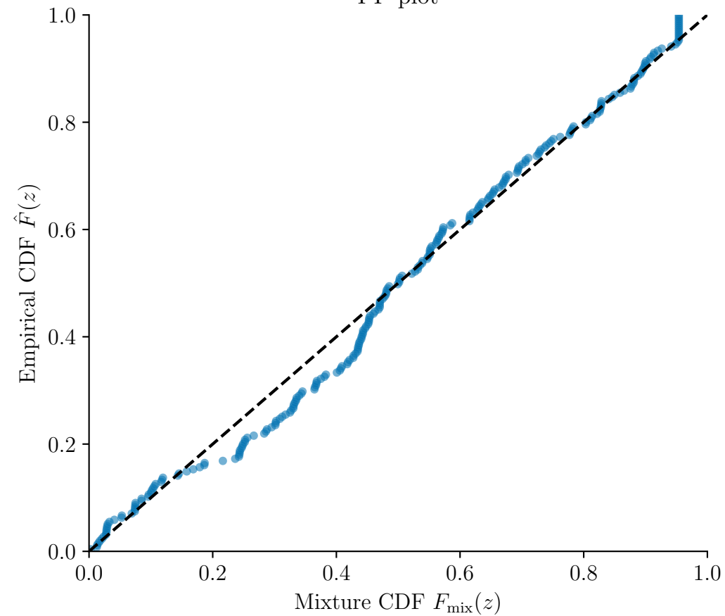
PP plot
