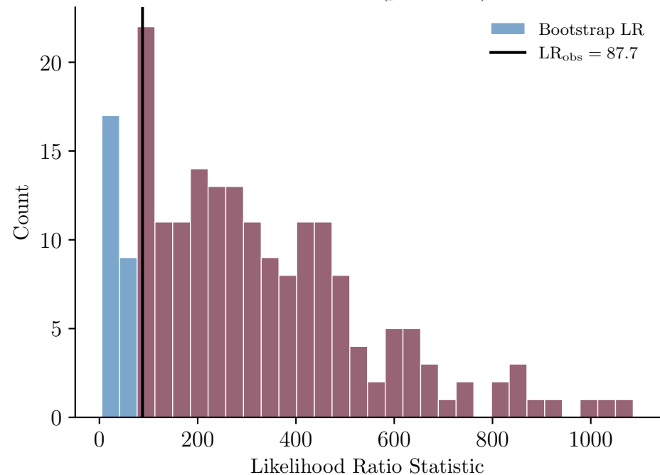
K=2 vs K=3 ( p = 0.635 )
