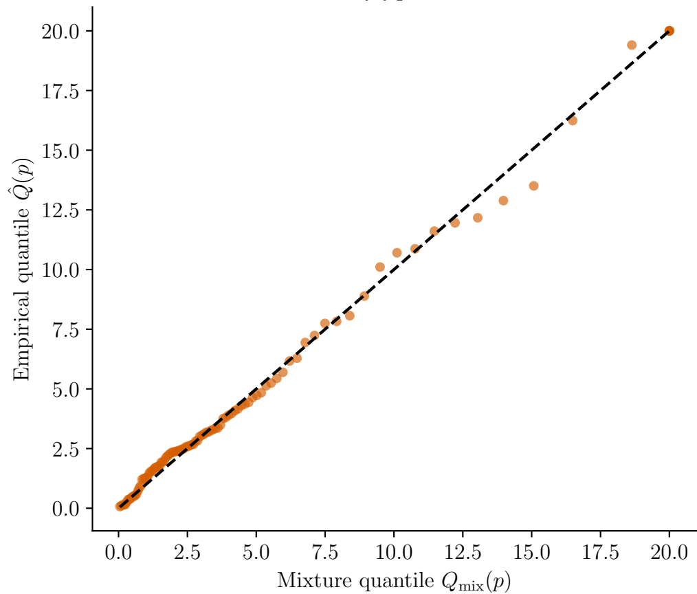
QQ plot
