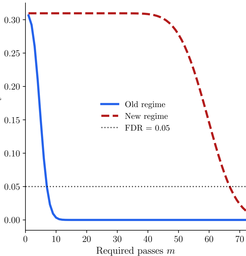
False discovery rate
