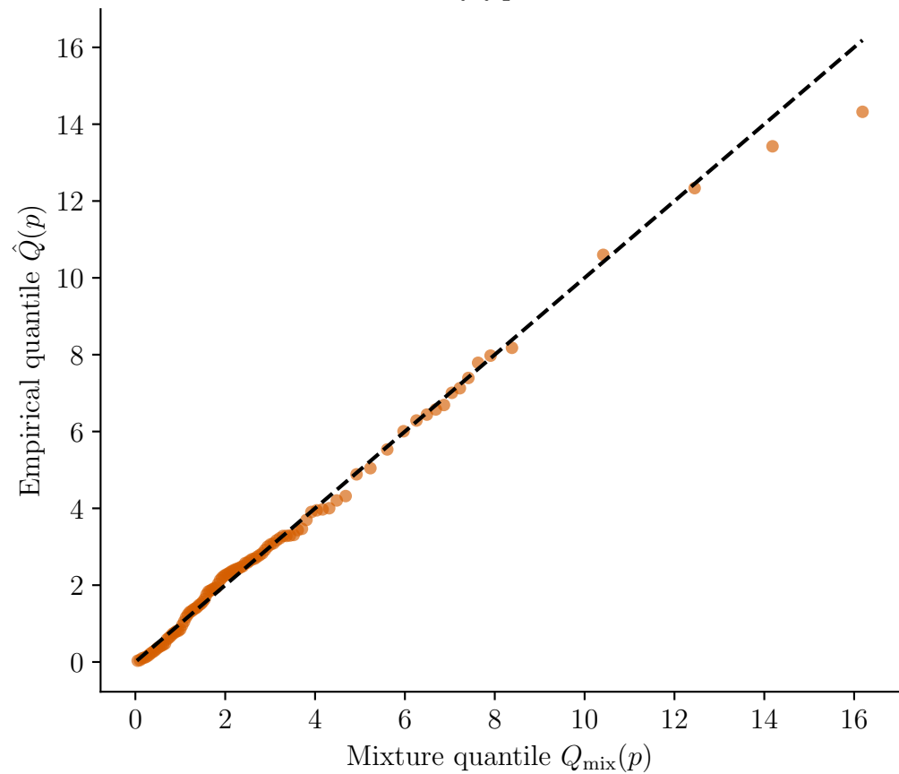
QQ plot
