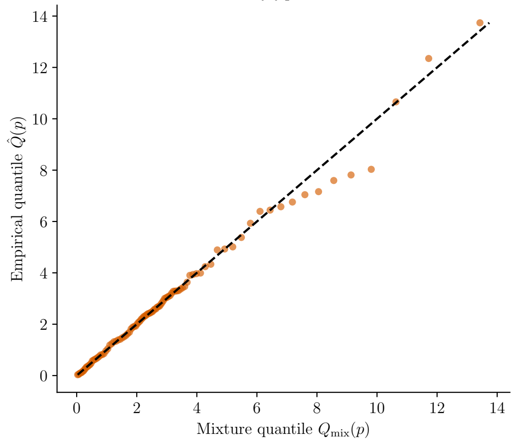
QQ plot
