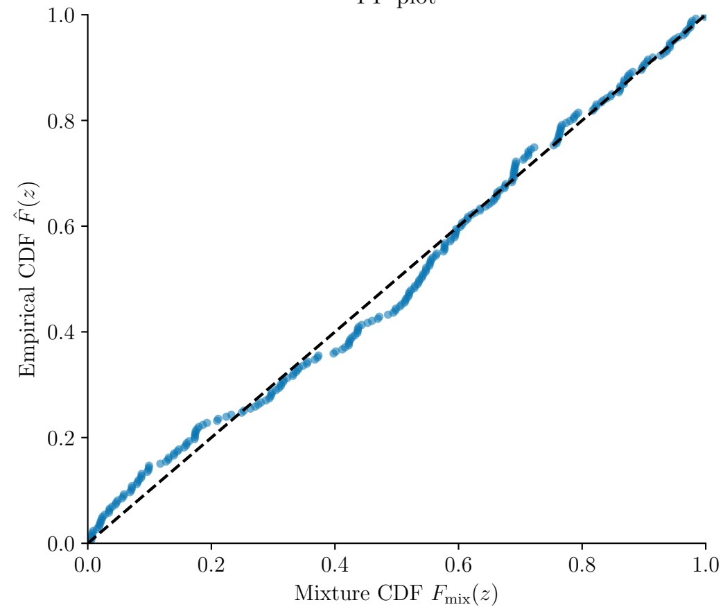
PP plot
