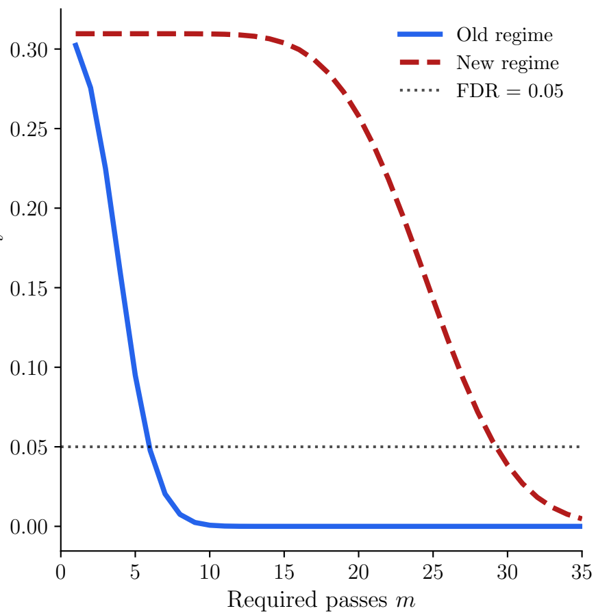
False discovery rate
