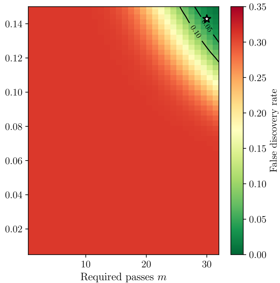
Cost ratio \lambda
