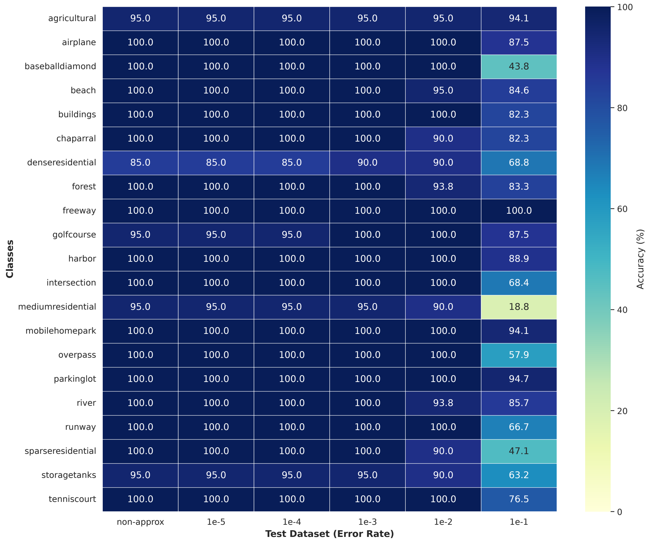
Accuracy Heatmap by Class — Model Trained on: 1e-3
