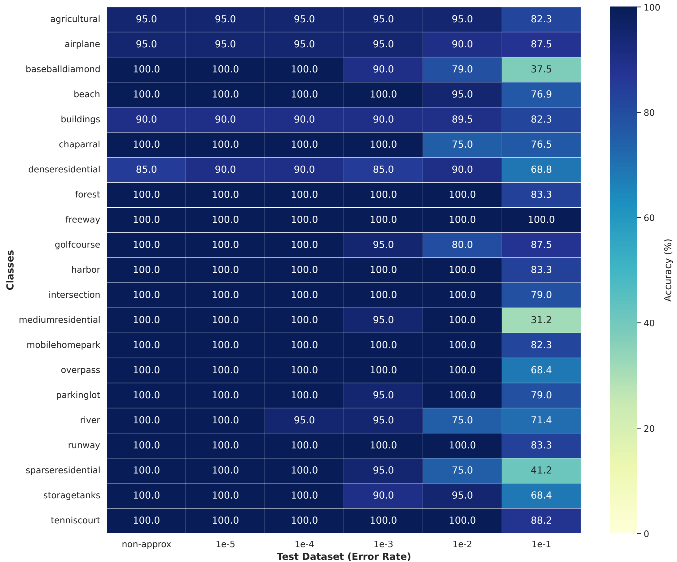
Accuracy Heatmap by Class — Model Trained on: non-approx
