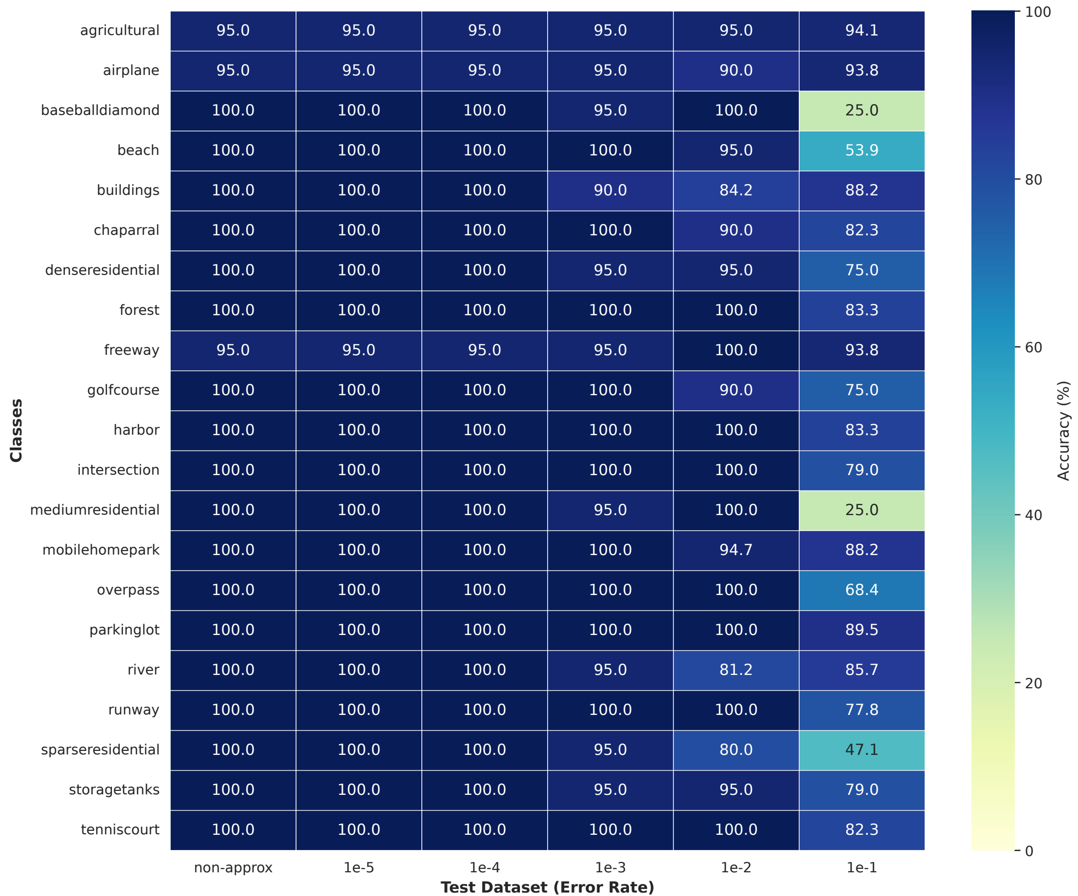
Accuracy Heatmap by Class — Model Trained on: 1e-5
