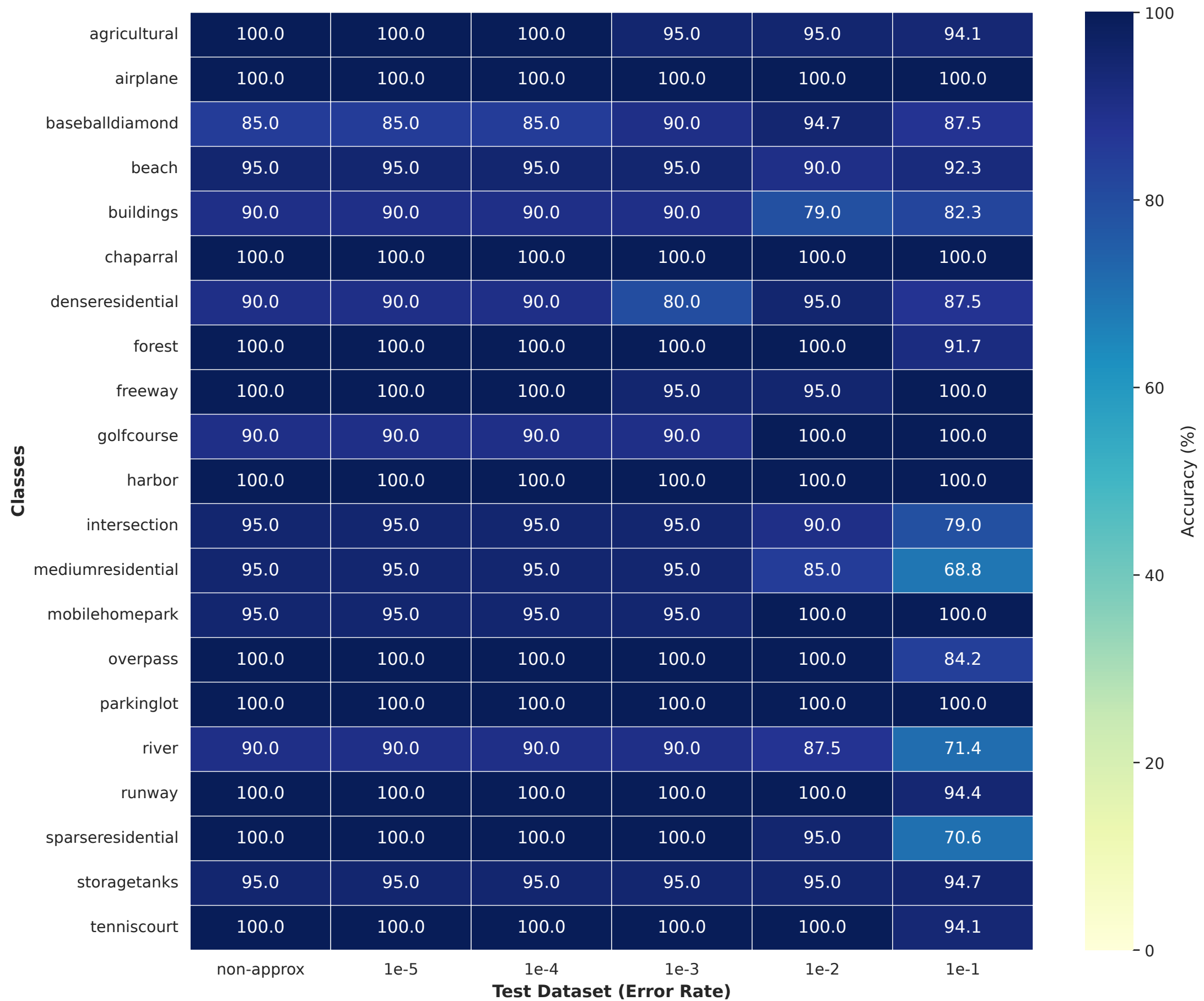
Accuracy Heatmap by Class — Model Trained on: 1e-1
