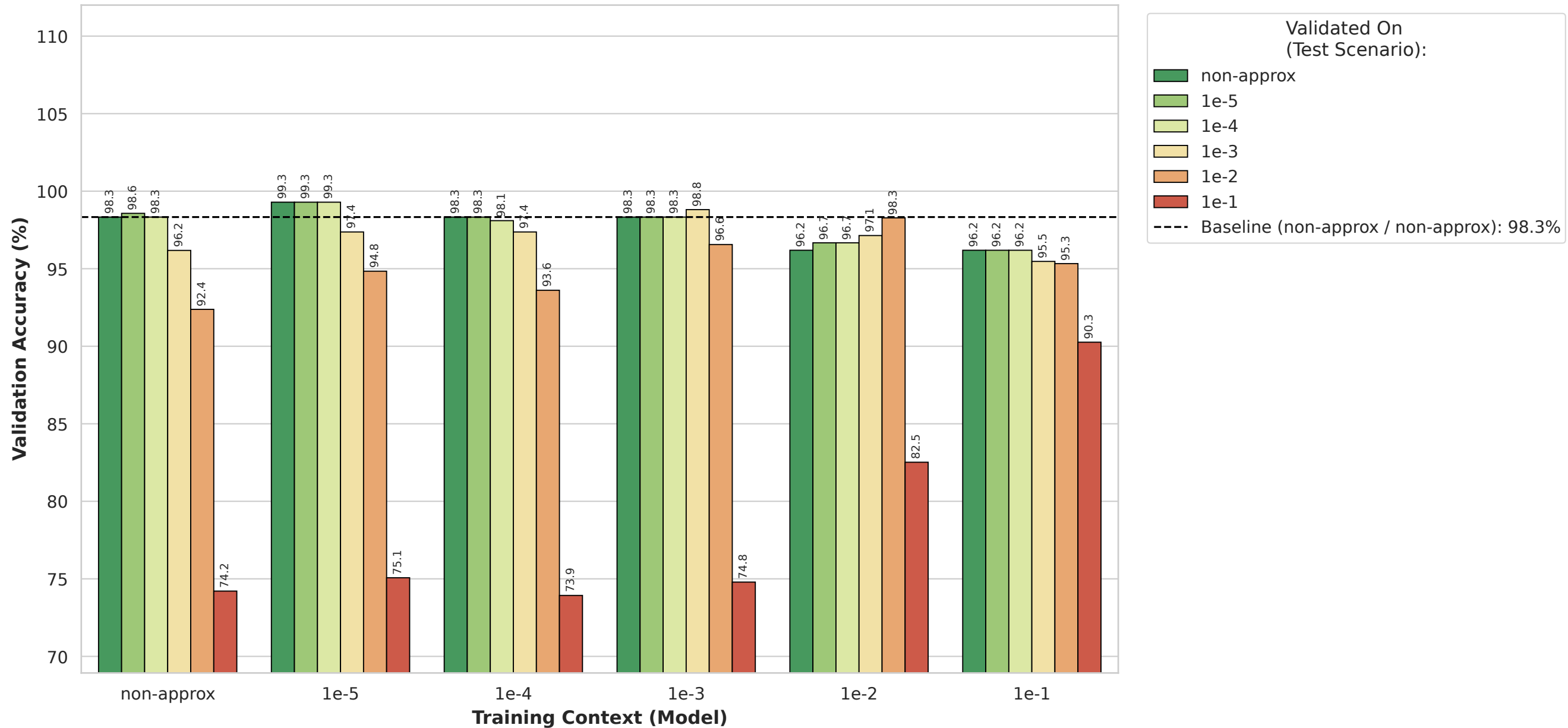
Cross-Validation Performance: Training Context vs. Test Scenarios
