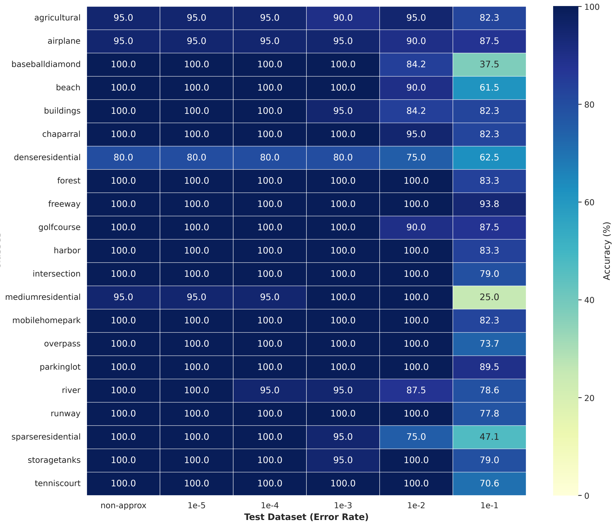
Accuracy Heatmap by Class — Model Trained on: 1e-4
