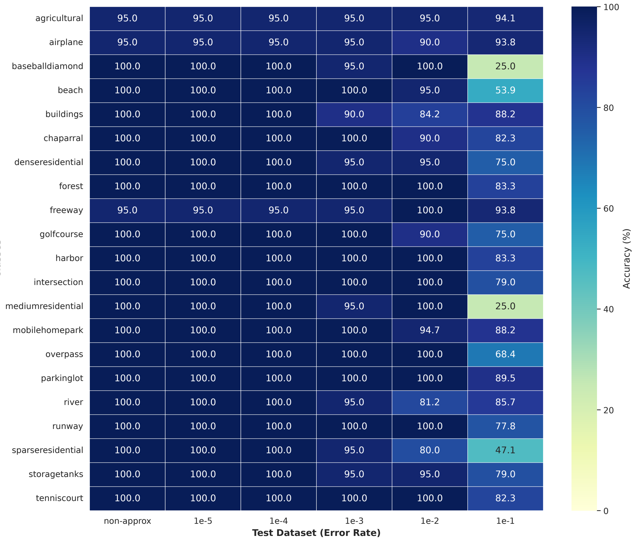
Accuracy Heatmap by Class — Model Trained on: 1e-5
