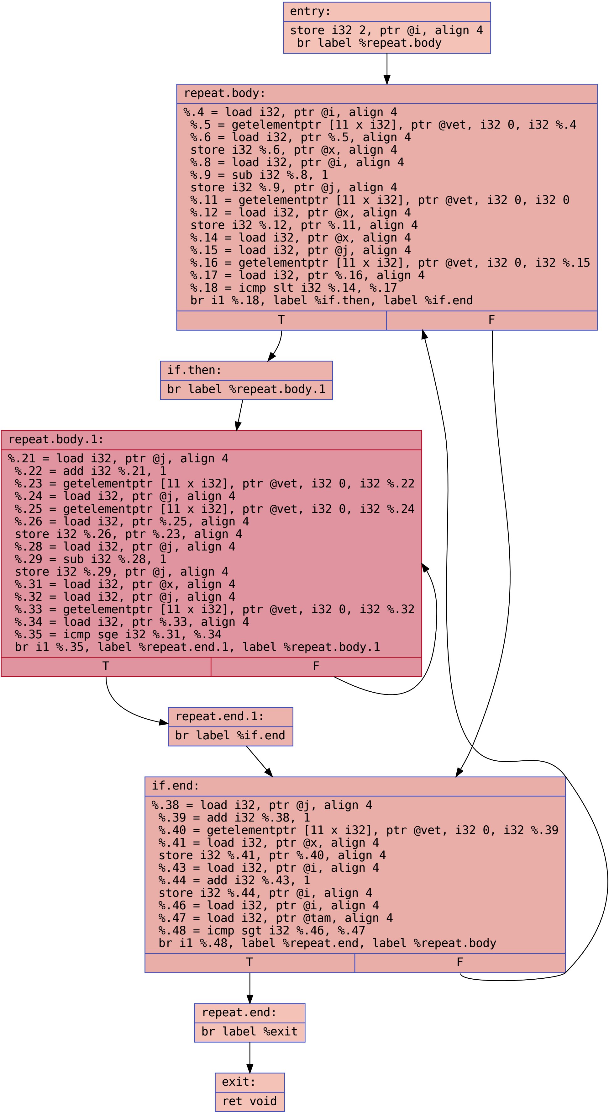
CFG for 'insert_sort' function
