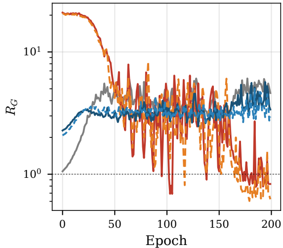
(c) Minority/majority grad. ratio
