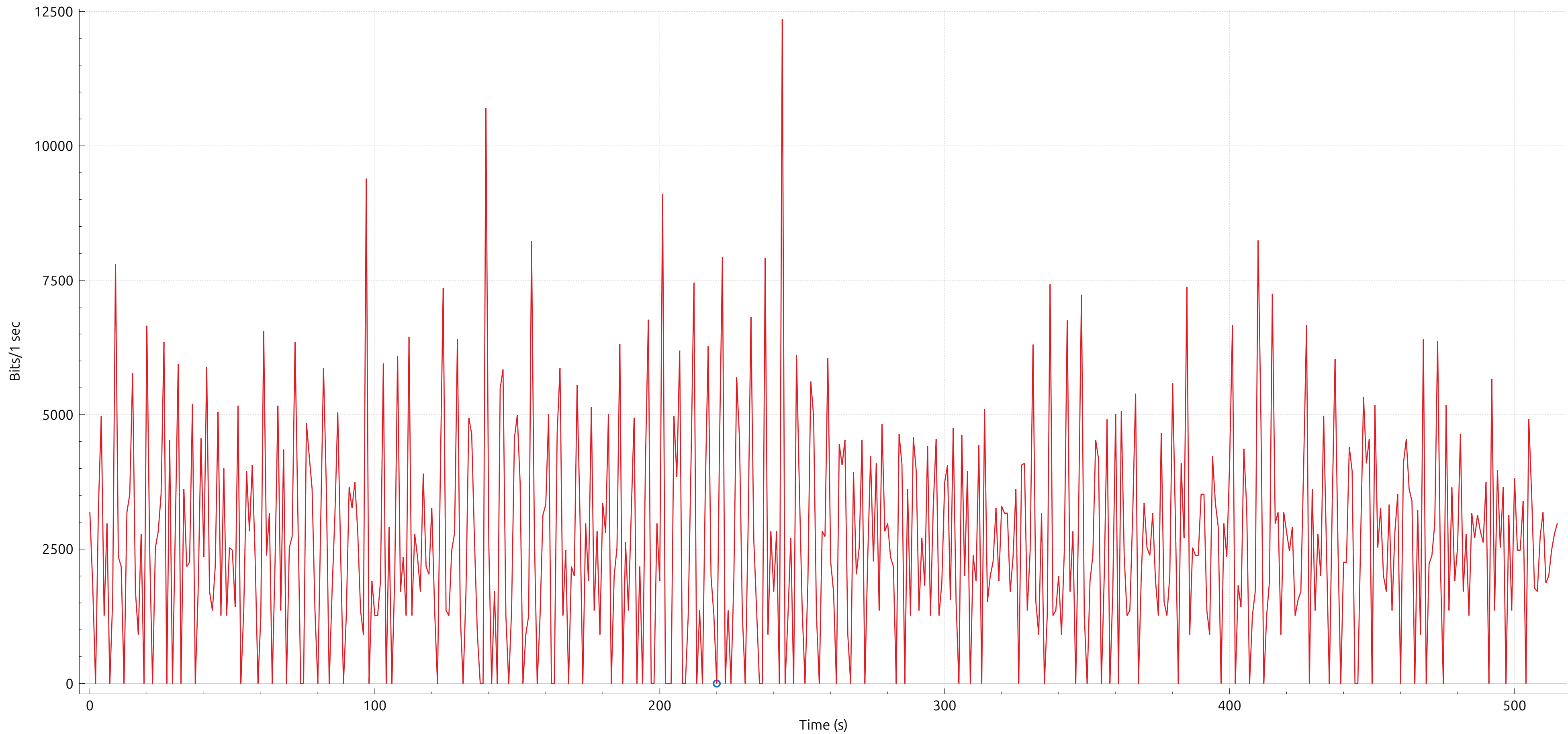
Wireshark I/O Graphs: capture-2.5-h2.pcapng
